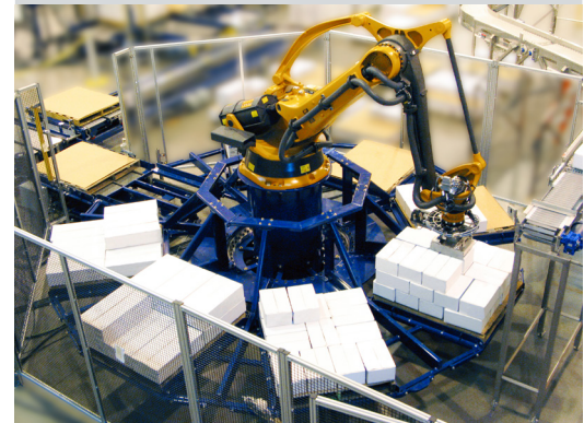
Robot putting a specific SKU on right pallet on turntable
