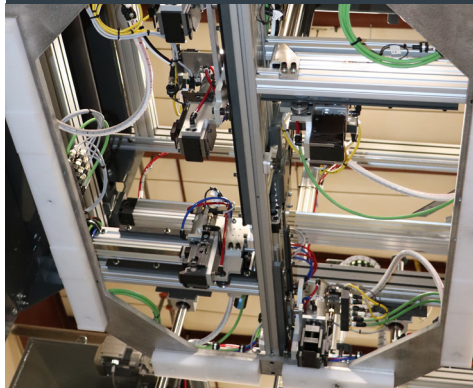
Destrapping cutting head assembly
