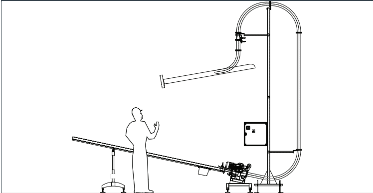
Drawing of Fleetwood Manual Can Lid Feeder with LLV Low Level V-Tray
